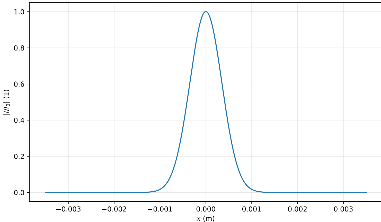
Intensity profile I(x, y = 0, z = 0.080m)/I_0 , P_{in}=0.4P_{cr} , artificial time
